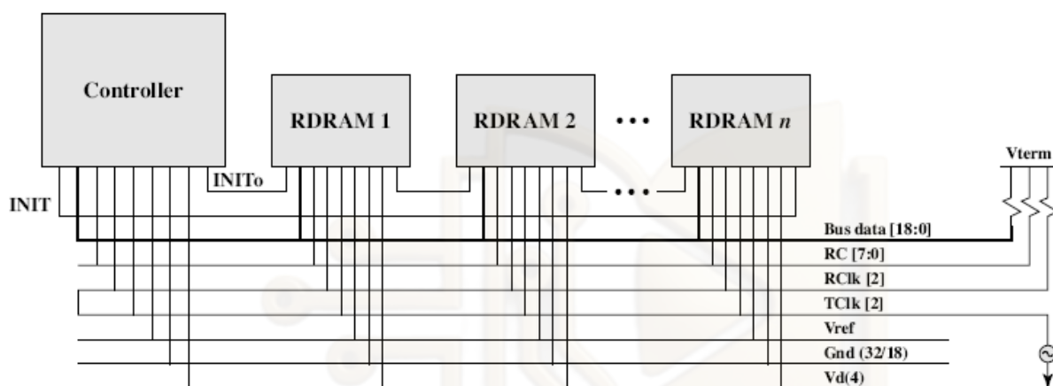
Figure 6.7: RDRAM Structure
