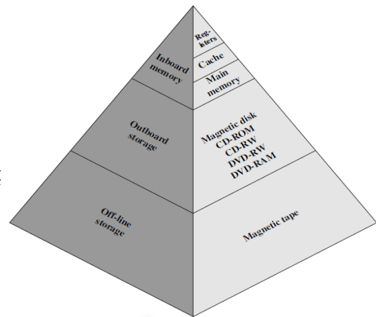
Figure 6.1: Memory hierarchy
