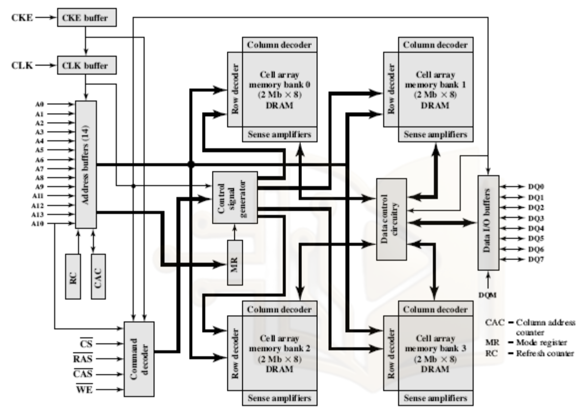
Figure 6.6: Synchronous DRAM
