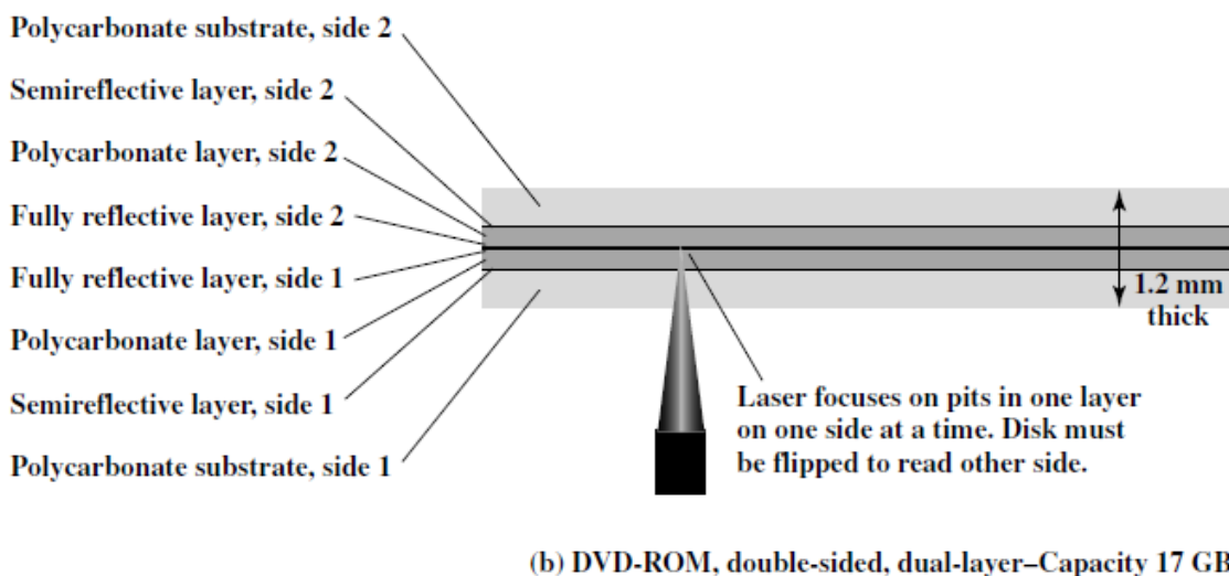
Figure 6.11: CD-ROM and DVD-ROM
